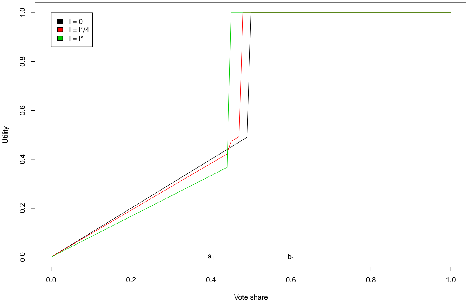
Utility function for a dominant party for different values of l
